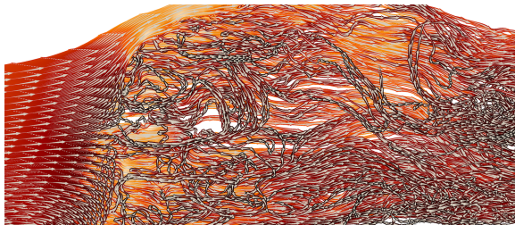
Figure 7: Streamlines depicted through light gray arrow shapes combined with a halos colored with a color map to depict velocity.
